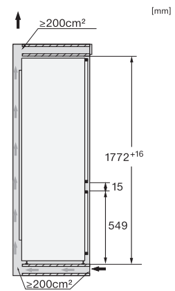
KF7742B, KF7742C, KF7742D, KF7772B, side view
