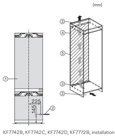
KF7742B, KF7742C, KF7742D, KF7772B, installation
