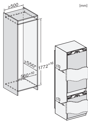
KF7742B, KF7742C, KF7742D, KF7772B, built-in
