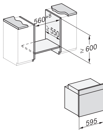
H226x-1B/BP/E/EP/VP, H2x6xB/BP, H7x6xB/BP/BPX, installation drawings
